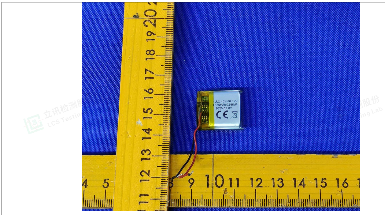
Details of: Battery View-1
