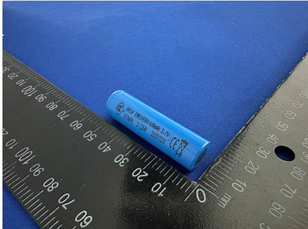
Picture 7. Side view-1 of cell for model HYLN IMR14500-600mAh
