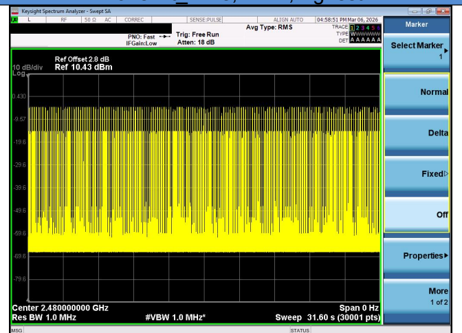
Transmit_Time,1DH1,Highest
